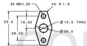
Oil Outlet
